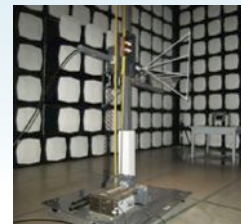
EMI shielding test
